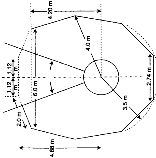
Cage for Hammer Only
